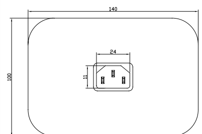
Connector Drawing
